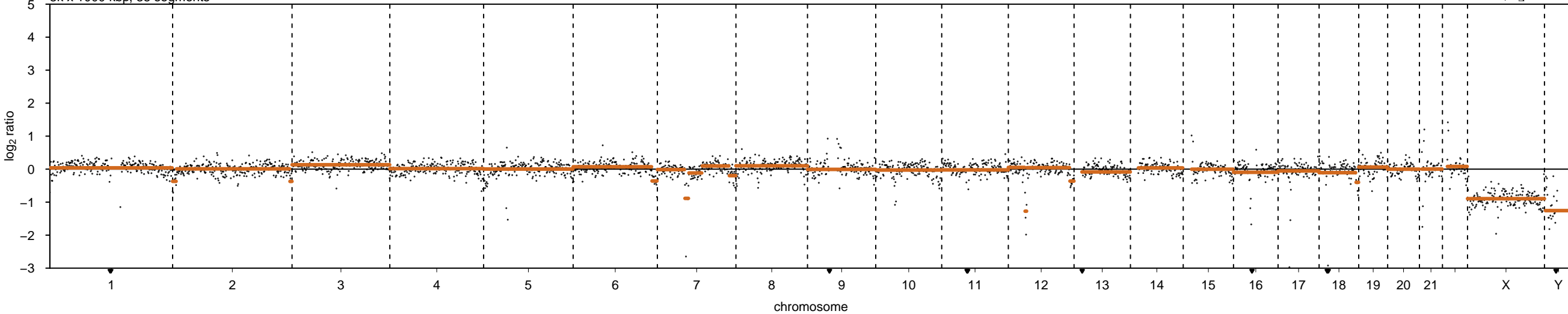
20241118_C5ABE8e_hEm75_4_WGS (56,790,571 reads)
