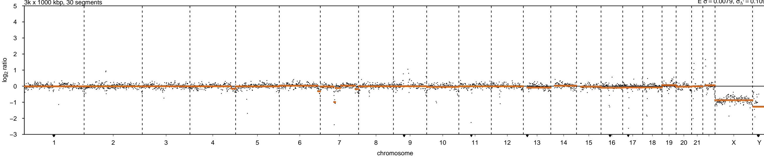
20241118_C5ABE8e_hEm75_3_WGS (46,063,852 reads)
