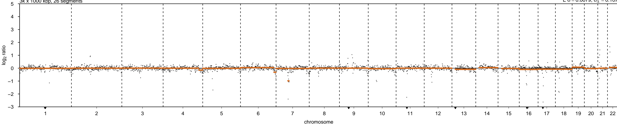
20241118_C5ABE8e_hEm75_3_WGS (46,063,852 reads)
