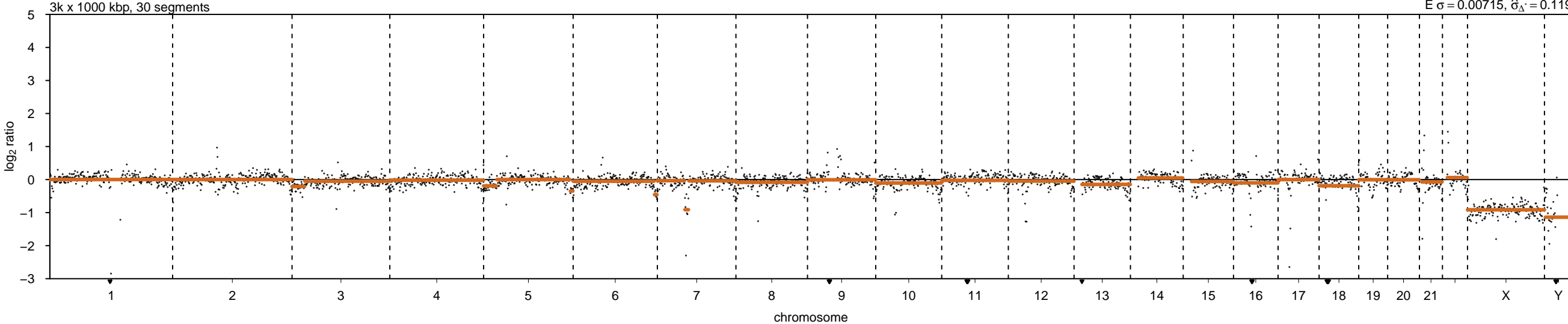
20241118_C5ABE8e_hEm75_1_WGS (56,154,880 reads)
