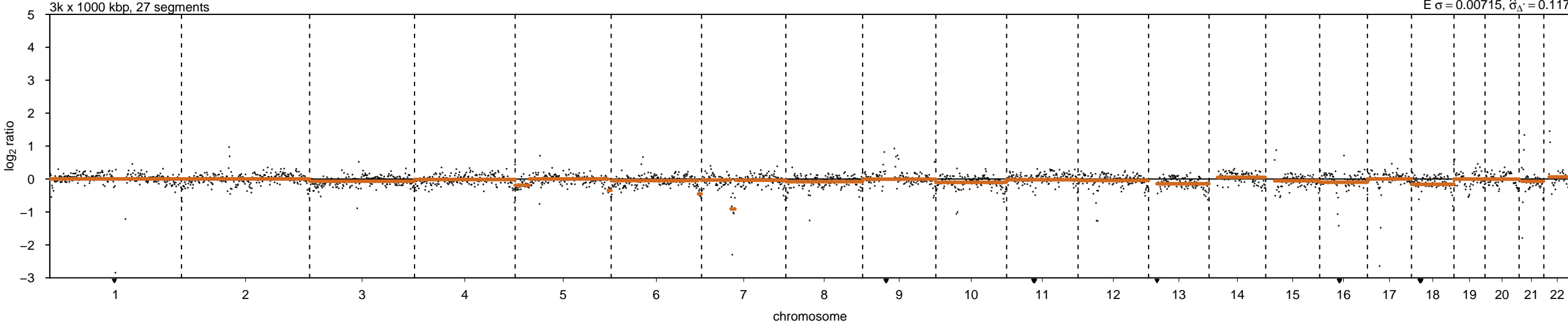
20241118_C5ABE8e_hEm75_1_WGS (56,154,880 reads)
