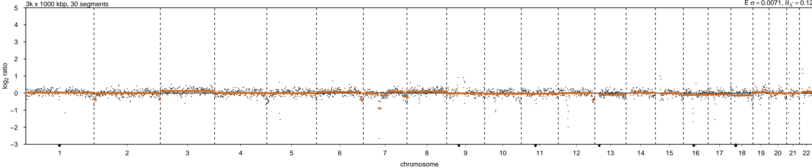
20241118_C5ABE8e_hEm75_4_WGS (56,790,571 reads)
